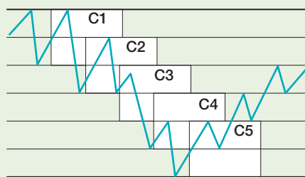
Cascade regulation
